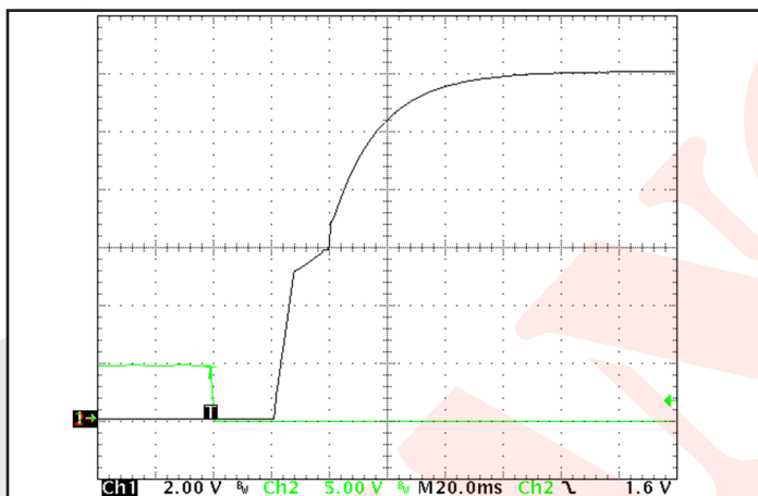
Figure 7: Typical startup waveform. Input voltage pre-applied, CH1: Vout (1V/div), CH2: ON/OFF (5V/div), Horizontal scale (20ms/div).
